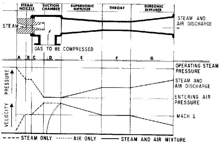
diagram of the pressure and velocity variations within a steam jet ejector handling air.
