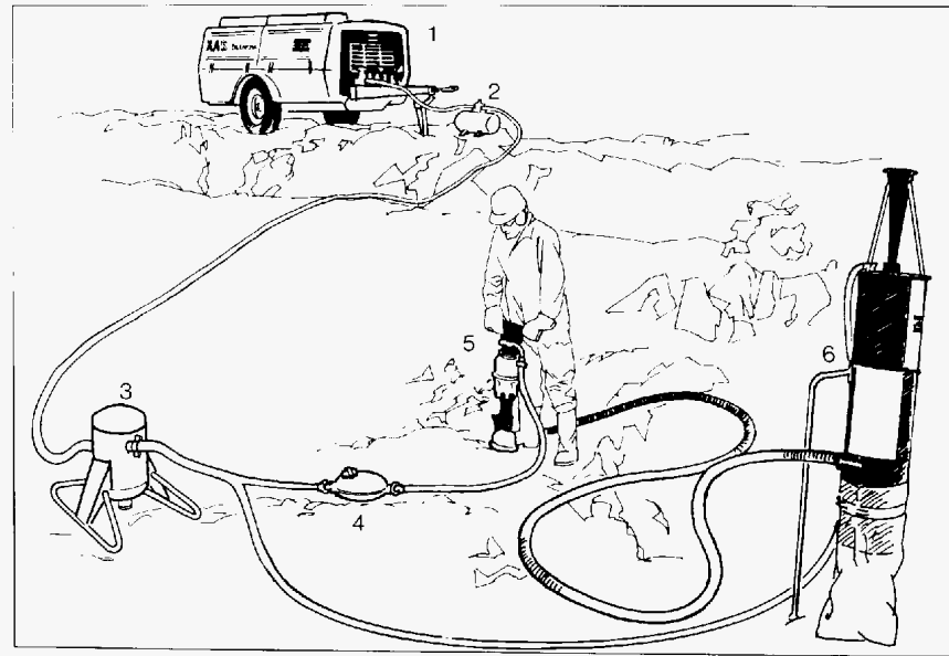
Fig. 8:3 Temporary air distribution for smaller-scale installation 1. compressor 3. water separator 5. silenced breaker 2. alcohol dispenser 4. lubricator 6. dust collector
