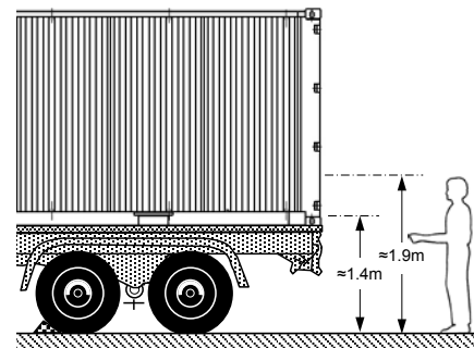
Figure 5.10 Seal heights - freight container
