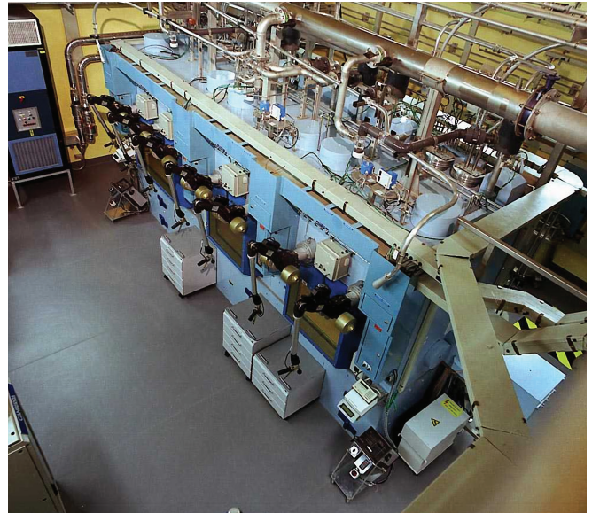
Euratom on-site laboratory at the reprocessing plant in La Hague (France) operated by the JRC.
