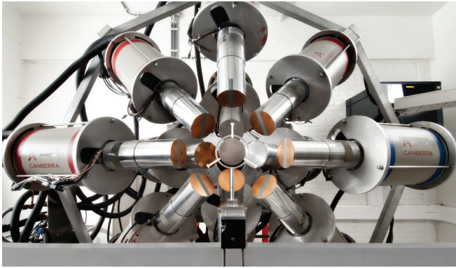
GAINS spectrometer for nuclear data measurements.
