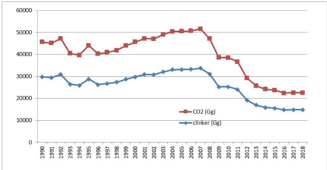
Figure 4.2 Trend of clinker production and CO 2 emissions 1990-2018 (Gg)
