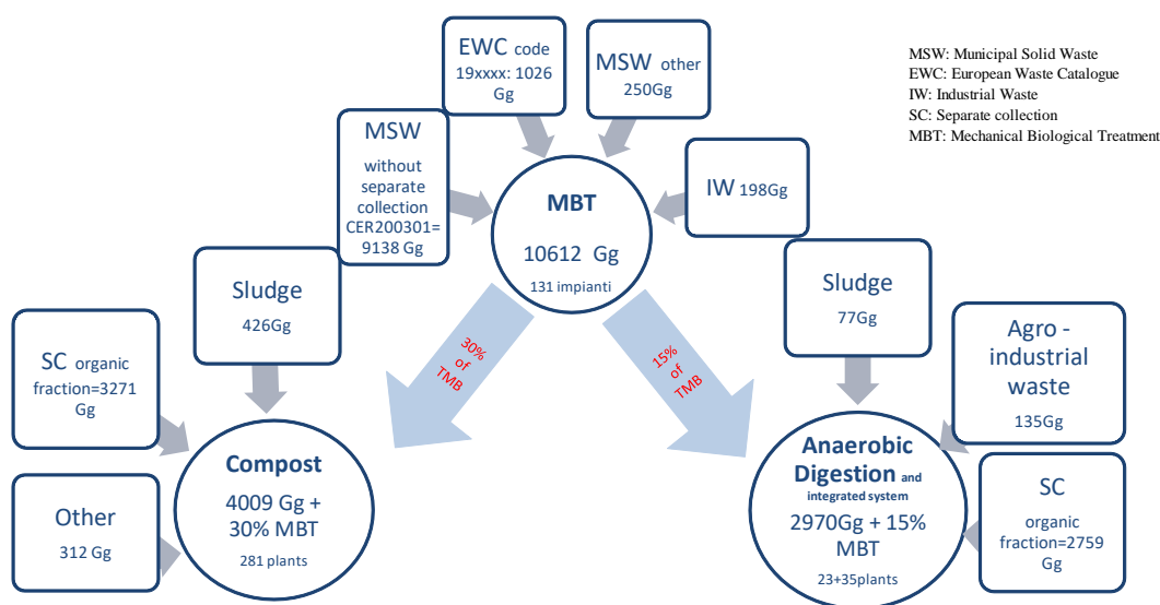
Figure 7.4 Waste treated in compost and anaerobic plants in 2018
