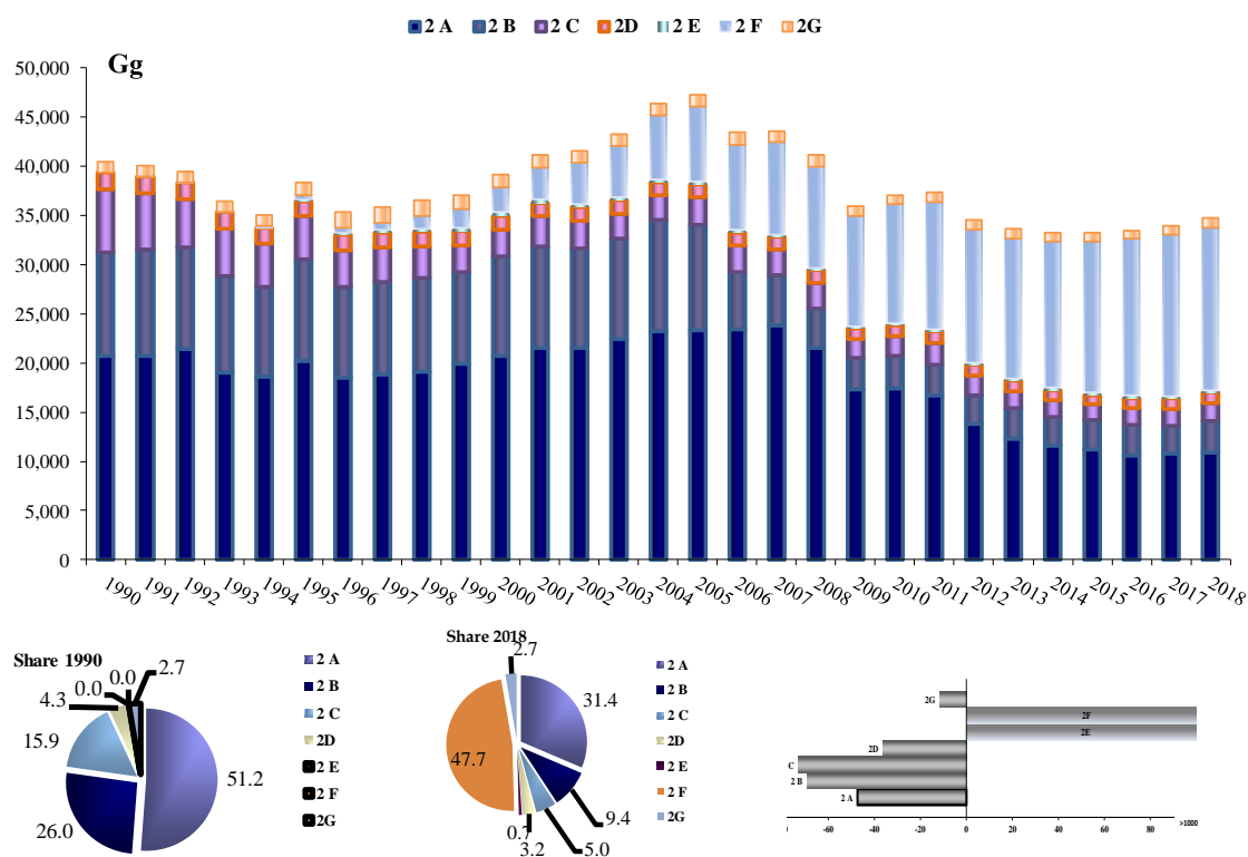
Figure 2.9 Trend of total emissions from the industrial processes sector (1990-2018) (Gg CO 2 eq.)
