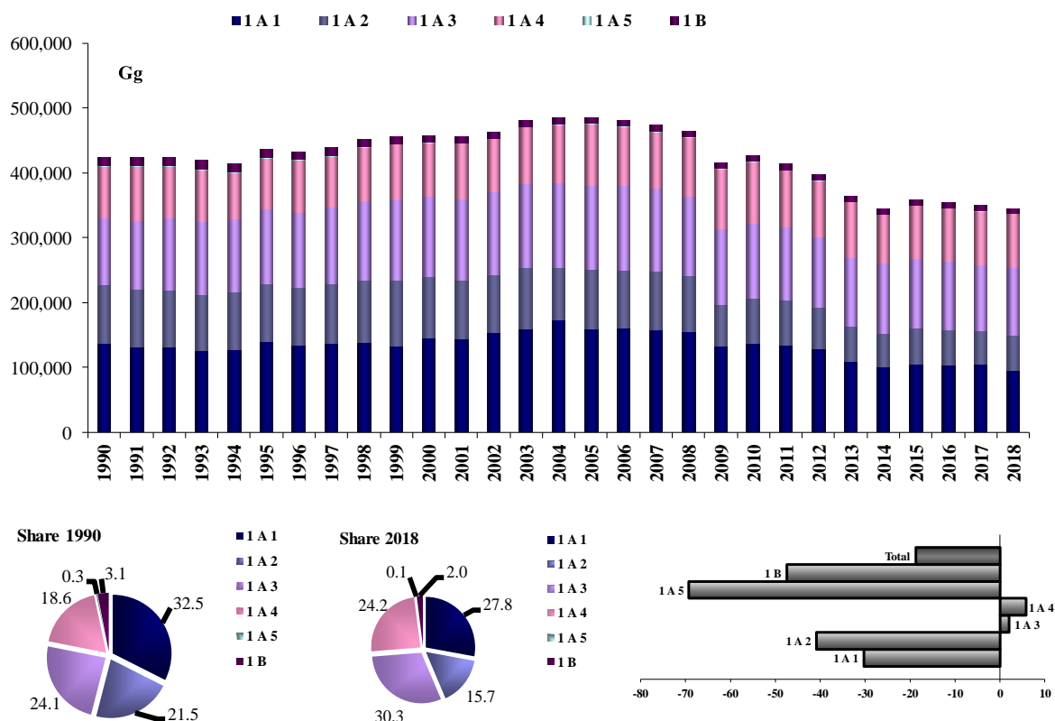
Figure 2.8 Trend of total emissions from the energy sector (1990-2018) (Gg CO 2 eq.)
