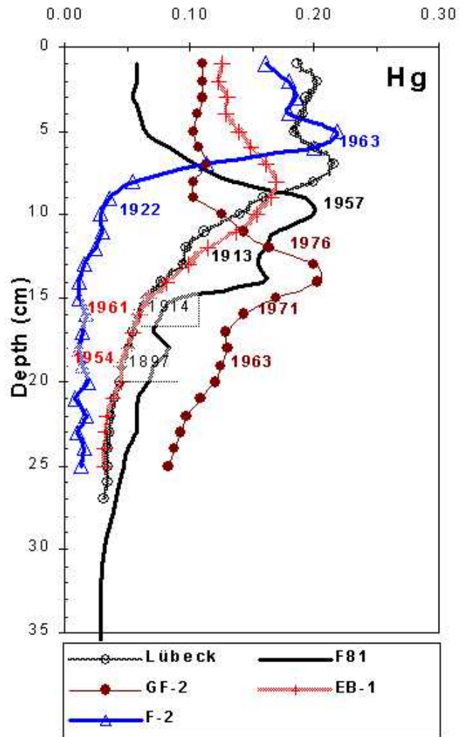
Figure 6.11 Vertical distribution of mercury (mg/kg dry-weight basis) in sediment from Lübeck Bay, Gdansk Bay, Gulf of Finland (GF-2), Bothnian Bay (F-2) and Bothnian Sea (EB-1) in 1993. The age of the sediment is indicated. Figure from HELCOM (2001), original presented courtesy of HELCOM, Finland.
