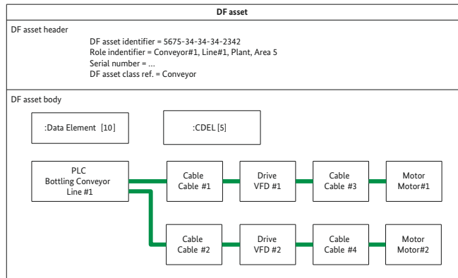
Figure 9 – Example of composite DF asset body
