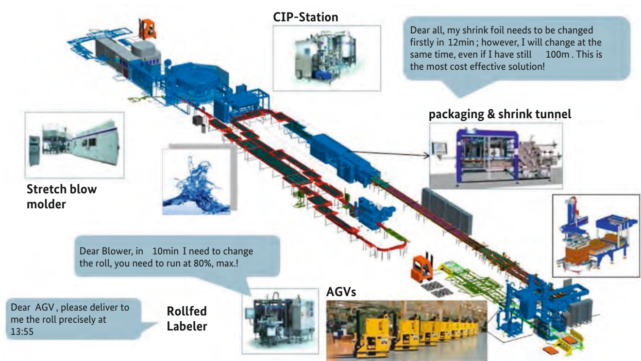
Figure 9 – Use case buffer-free-filling
